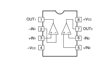
IC5, 801: NJM2068MD-TE2 Dual operational amplifier
