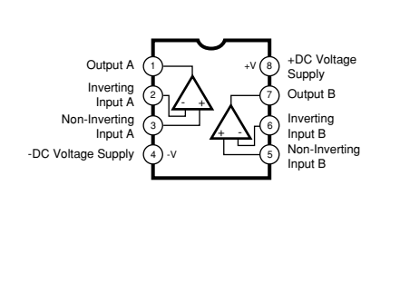
IC2: NJM3404AM-TE1 Single-supply dual operational amplifier
