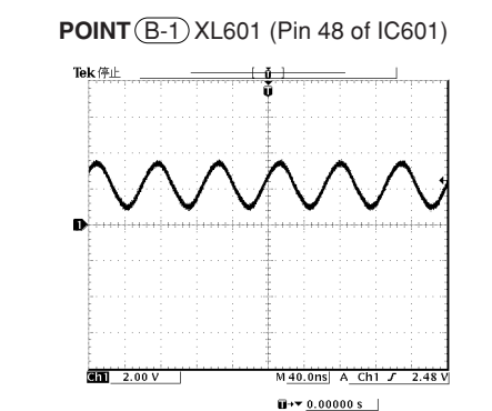
IC601, 602: YDA141-SZ Sound projector
