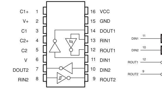
IC6: MAX3232CDWR 3-V to 5.5-V multi-channel RS-232 line driver/receiver
