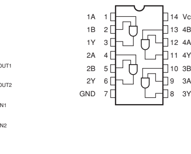
IC7: TC74HC08AF Quad 2-input AND gate
