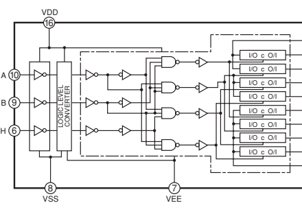
IC4: TC4052BF Analog multiplexer/demultiplexer
