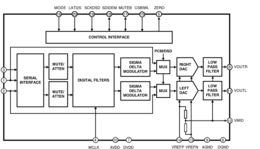
IC603: WM8728 24-bit, 192 kHz stereo DAC
